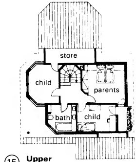
15 Upper floor → 14
